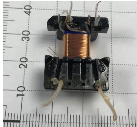
Primary winding with tubing
