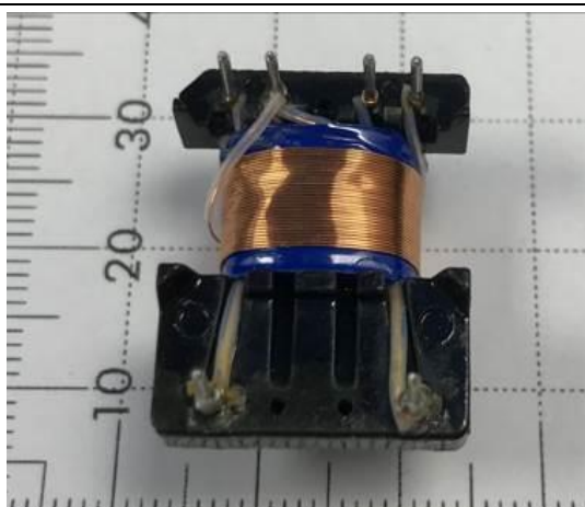
Primary winding with tubing
