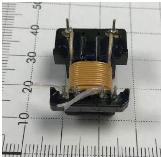
Secondary TIW winding with tubing
