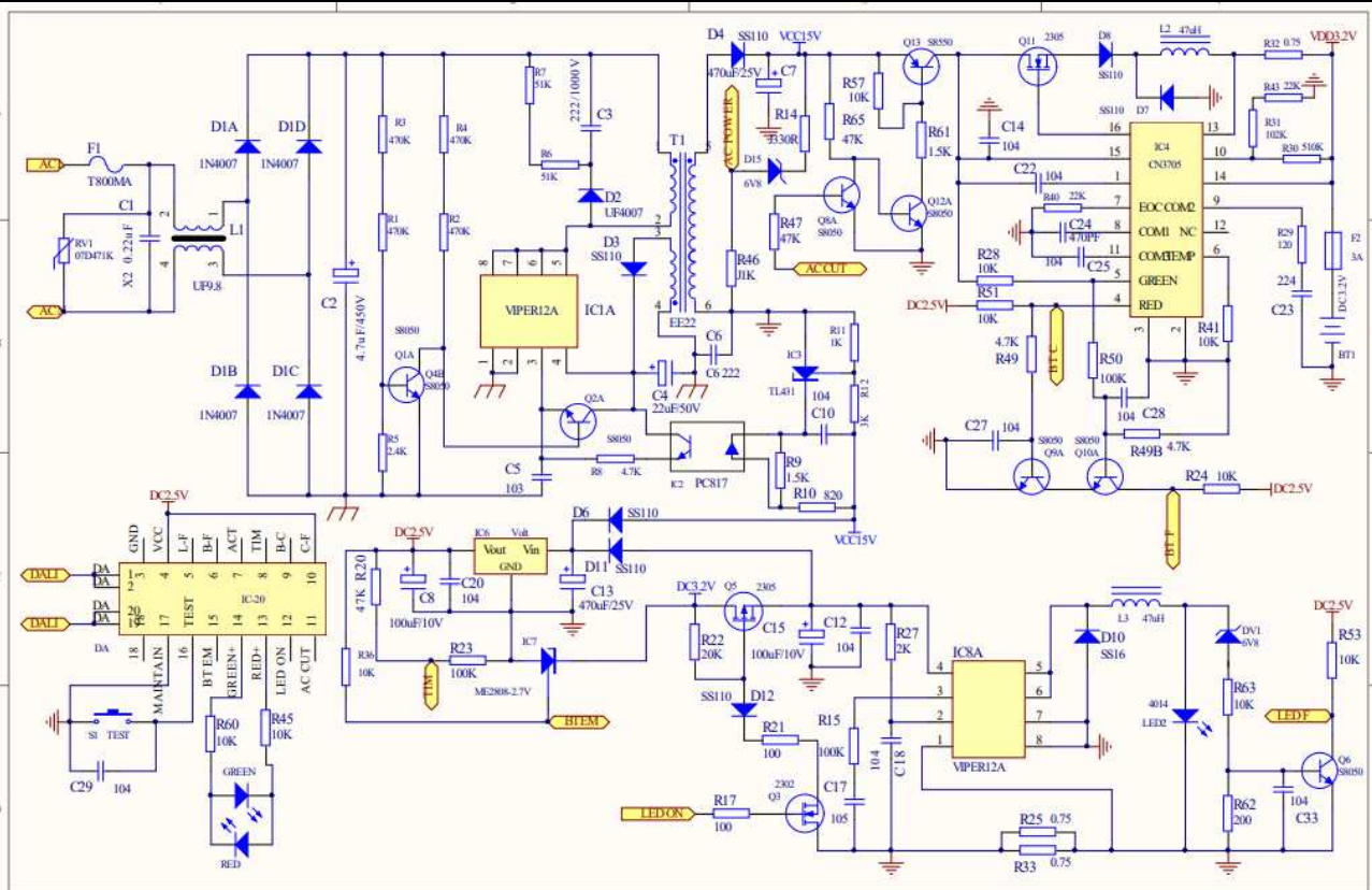
Circuit diagram
