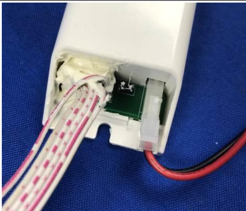
Output terminal with wire link for SPaaaabb-D63
