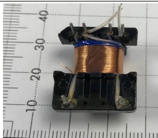
Primary winding with tubing
